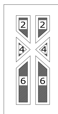
Drina
